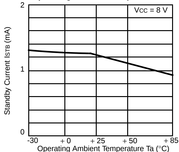
Fig. 25 -Standby Current vs. Operating Ambient Temperature
