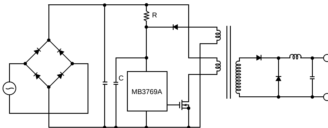
Fig. 8 - MB3769A Primary Control
